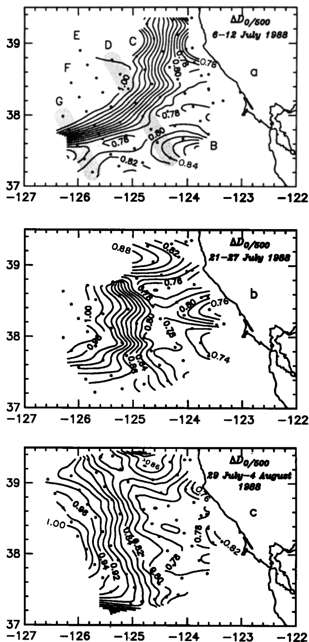
Fig. 6. Fields of dynamic height anomaly relative to 500 dbar from three surveys in 1988 (contour interval is 0.02 dyn m): (a) July 6–12; (b) July 21–27; (c) July 29–August 4. The shading and letters indicate sections shown in Figure 9.
