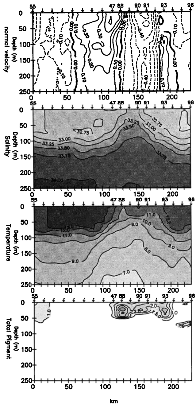
Fig. 8b. As in Figure 8a for a section along the northwest border of the survey on May 23-26, 1987. Stations 55-96 form an alongshore transect along the line farthest from shore (see Fig. 3), with the viewer looking offshore. The velocity is the component normal to the transects, defined to be positive shoreward.
