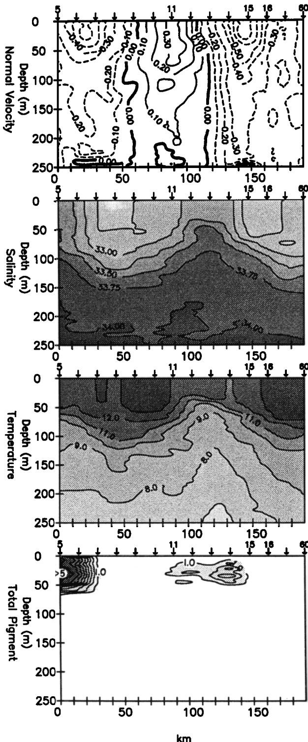
Fig. 8c. As in Figure 8a for a section along the southwest border of the survey on June 10, 1987 (see Figure 3).
